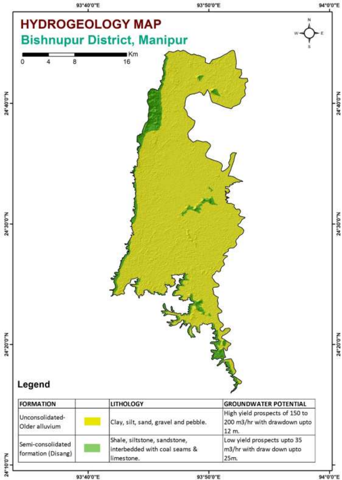
Fig.7a Hydrogeological map of the study area
