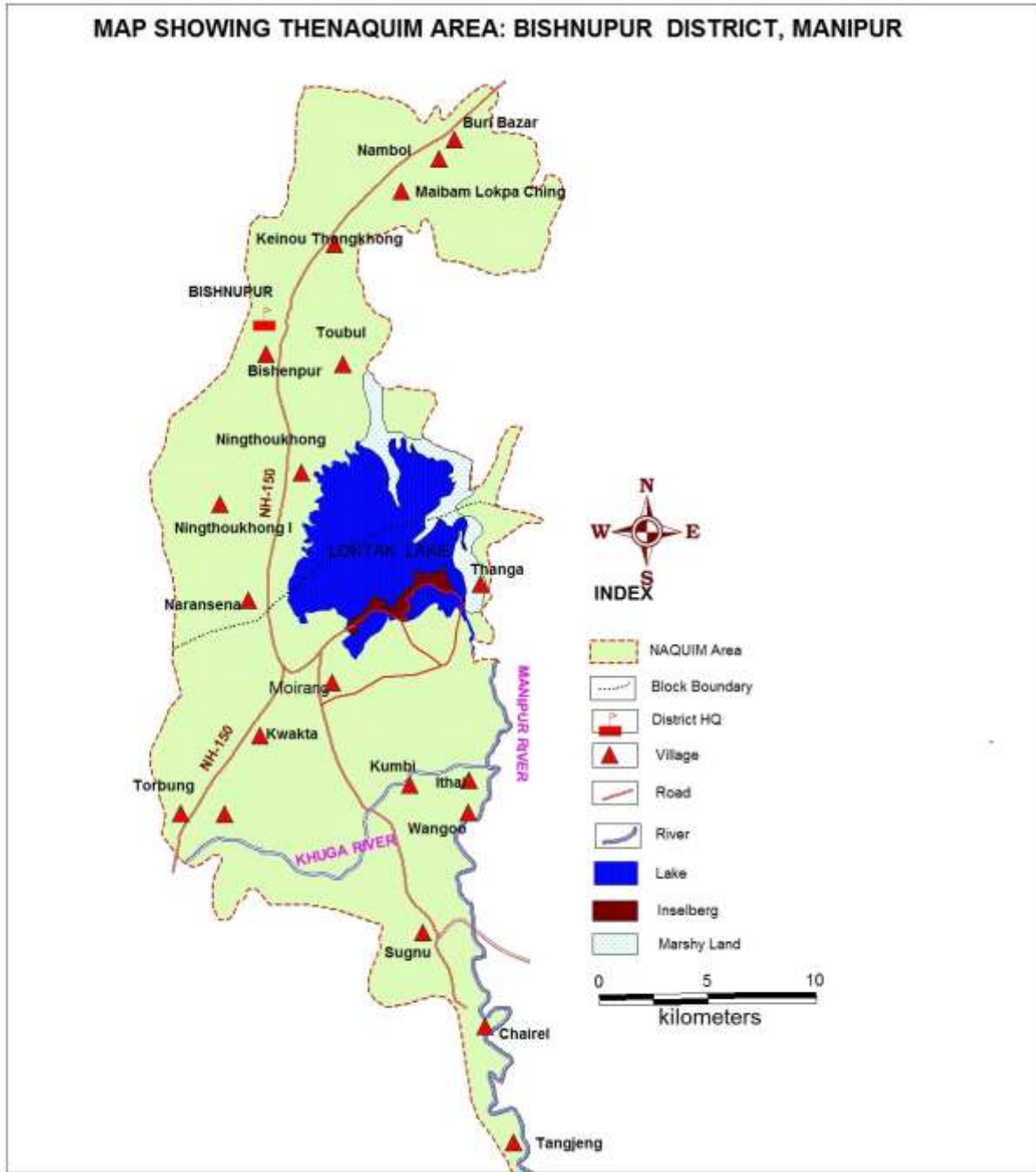
Fig.1 Map showing the study area: Bishnupur district, Manipur
